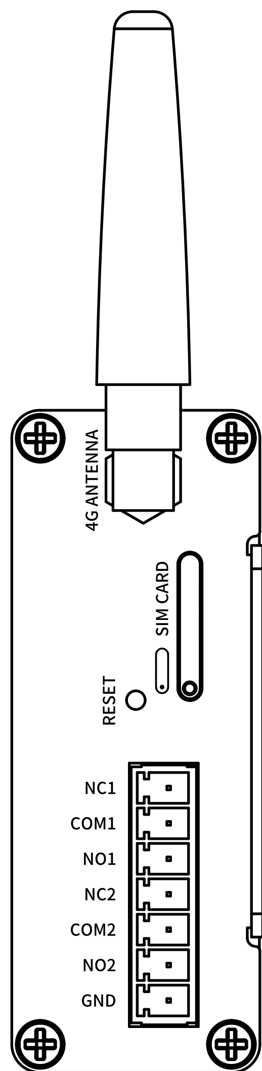
2 RIGHT VIEW
