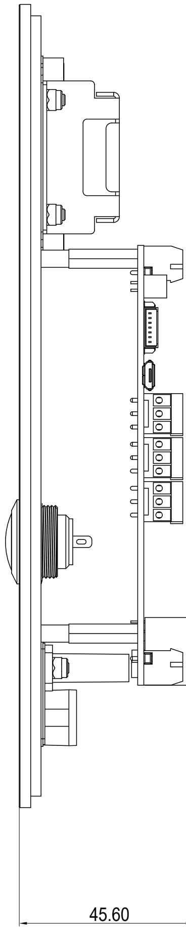
3 LEFT VIEW
